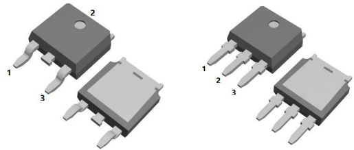
TO-252-2L 6N70G
